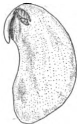
FIG. 267. — Embryo of Lima Bean, as it appears without the seed coat, and on removal of one cotyledon; \times \frac{1}{2} . The largest part is cotyledon.
